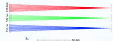
DIFFRACTIVE ACHROMATIC LENS
